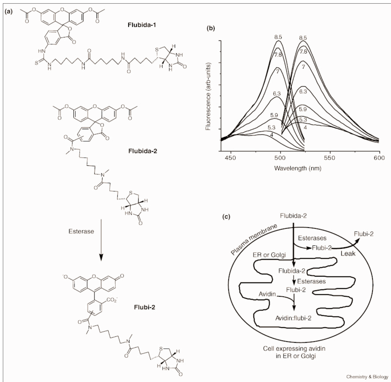
The pH-dependent fluorescence of flubi-2 and a strategy for targeting pH-sensitive dyes to organelles. (a) Chemical structures of Flubida-1, Flubida-2 and Flubi-2. (b) The pH dependence of Flubi-2's excitation (emission = 530 nm) and emission spectra (excitation = 480 nm). (c) A strategy for targeting Flubi-2 to the ER and Golgi compartments.
